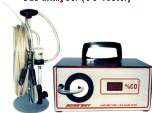
436-020 Digital CO Tester Portable CO tester to test fuel injection and carburetor systems. 12 V operation.
