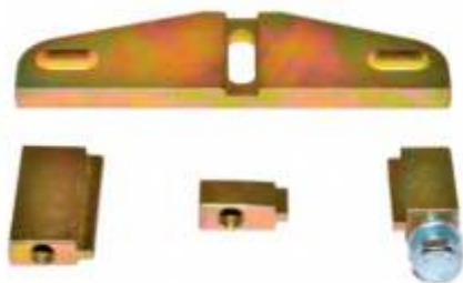
602-100 Flywheel lock Ford 1.25 1.4 1.6 1.7 1.8 2.0 2.2
