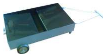
Oil drain (Truck) Trolley type on wheels Code Capacity Size 720-020 60L 90x50x15cm 720-030 240L 150x80x20cm
