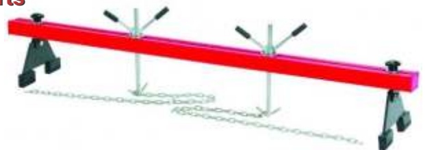
046-020 Engine support 500Kg capacity Engine support with double chain Length 1500mm
